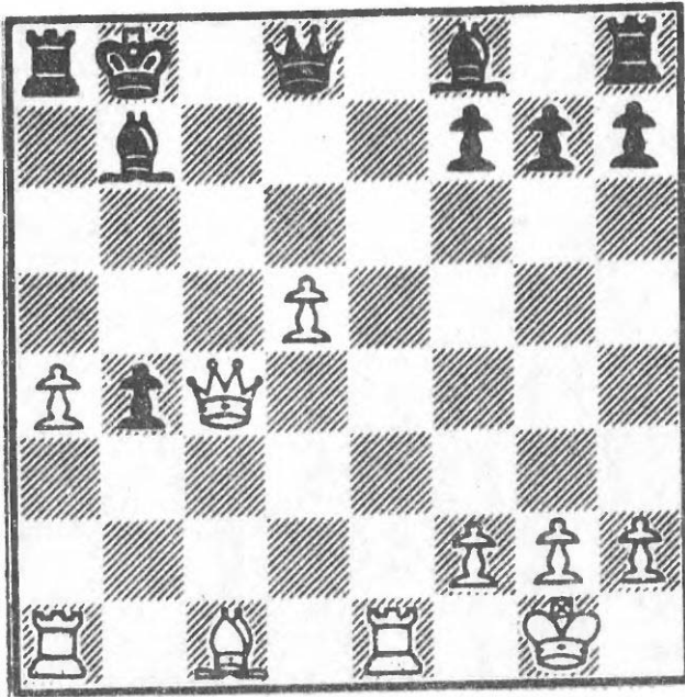
352 After 20...Kb8
